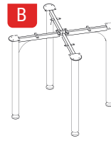
Bench Height Leg (with levelling feet) 900mm high
