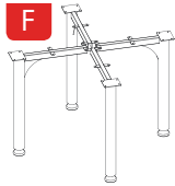
Fixed Height Leg (with levelling feet) 720mm high
