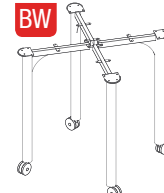
Bench Height Leg (with lockable castors) 970mm high
